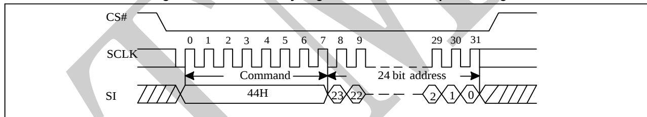
Figure 37. Erase Security Registers command Sequence Diagram
