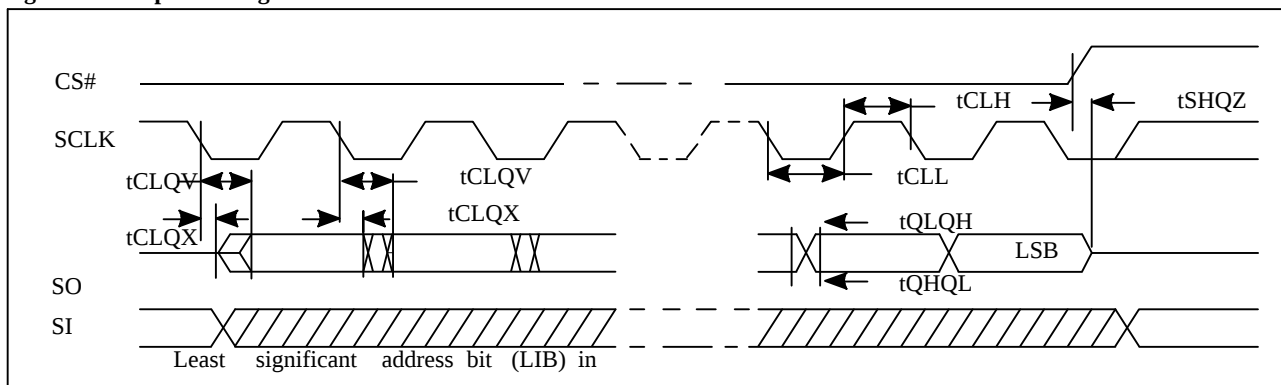
Figure 4-5 Output Timing
