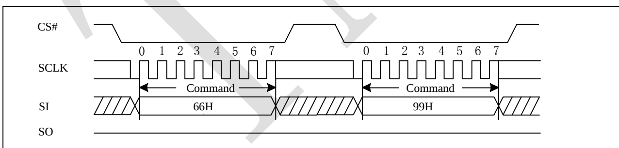
Figure 5-41 Reset Sequence
