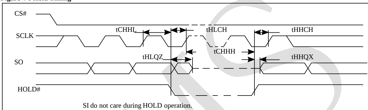
Figure 4-6 Hold Timing
