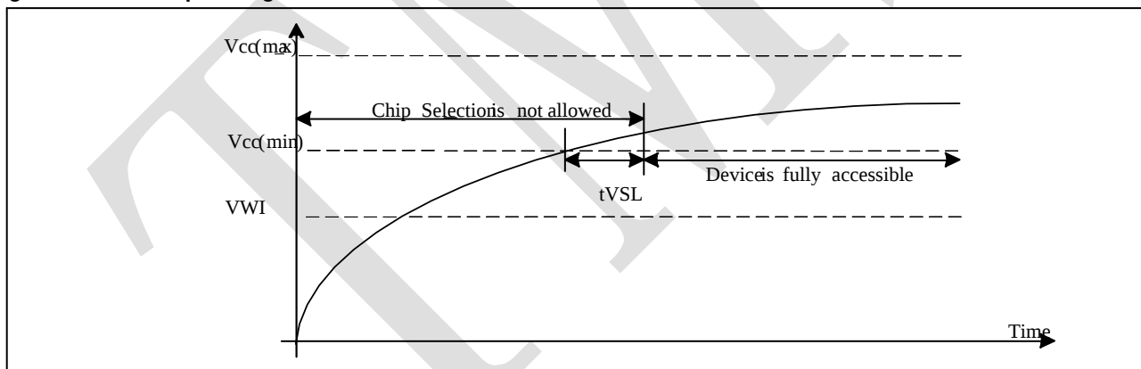
Figure 4-9 Power-Up Timing
