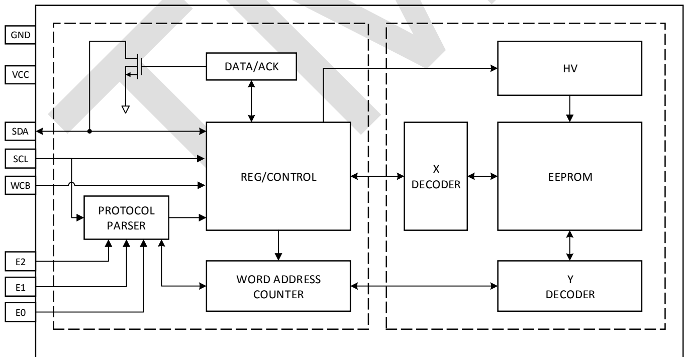
Figure 2-1 Block Diagram
