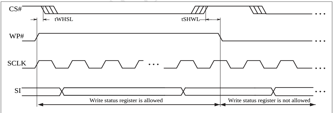
Figure 5-7 WP Timing
