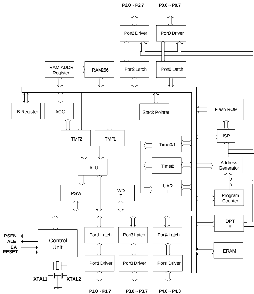
MG87FX52 Block Diagram
