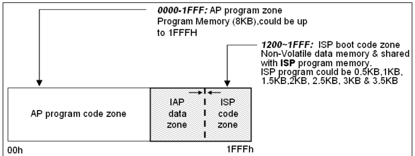
Address Space for MG87FEL52A embedded Flash memory
