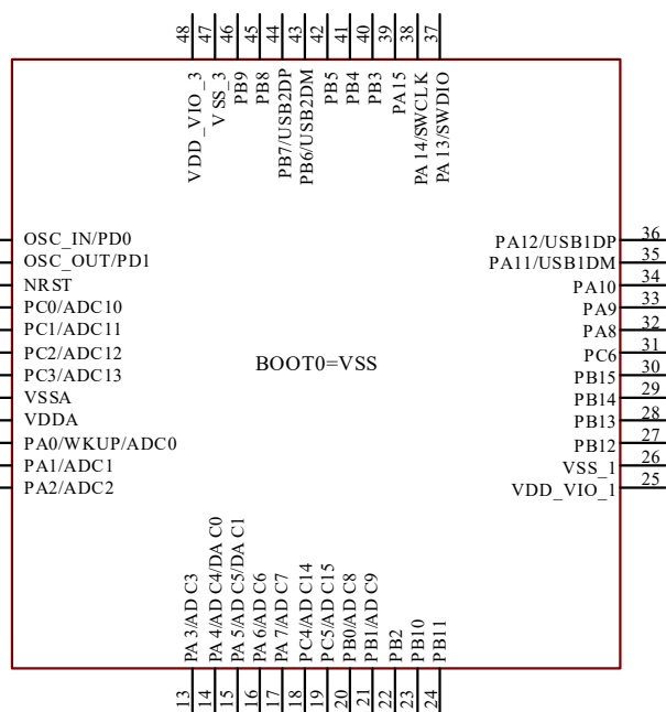
CH32V305CCT6
